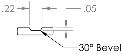
Rout Profile SCALE 1 : 1
