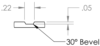
Root Profile SCALE 1 : 1
