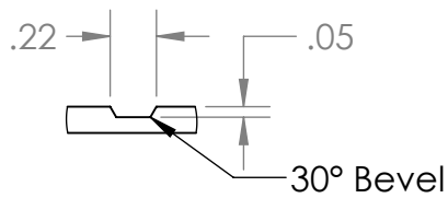
Rout Profile SCALE 1 : 1
