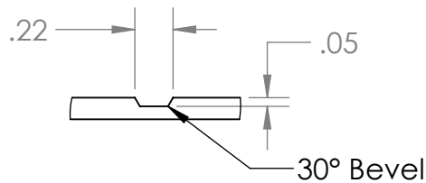
Root Profile SCALE 1 : 1
