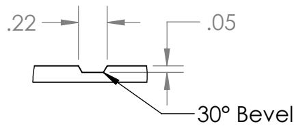
Rout Profile SCALE 1 : 1
