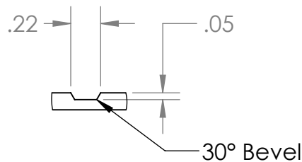
Rout Profile SCALE 1 : 1
