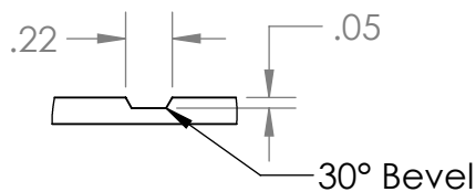
Rout Profile SCALE 1 : 1
