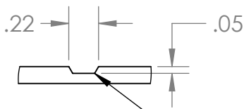
Rout Profile SCALE 1 : 1
