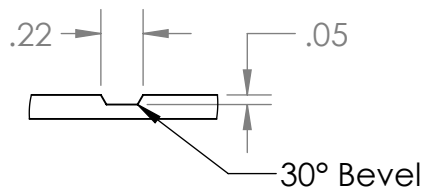
Rout Profile SCALE 1 : 1
