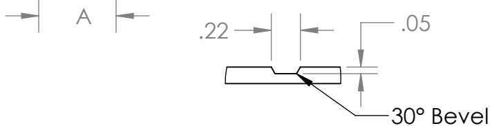
Rout Profile SCALE 1 : 1
