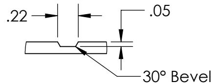
Rout Profile SCALE 1 : 1
