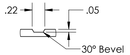
Rout Profile SCALE 1 : 1
